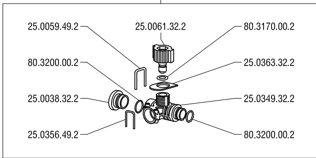
Kit by-pass intermedio 25.9861.97.3 Intermediate by-pass kit
