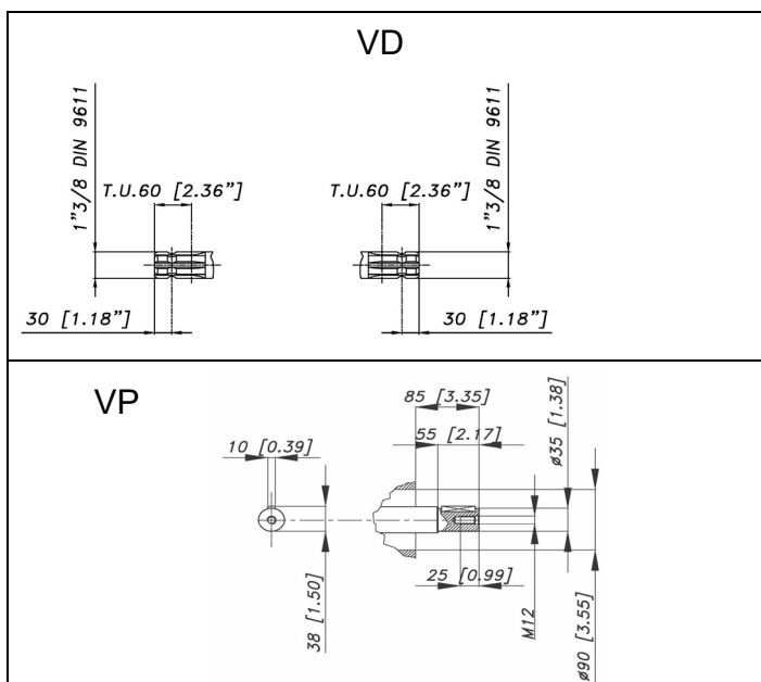
ALBERO POMPA - PUMP SHAFT
