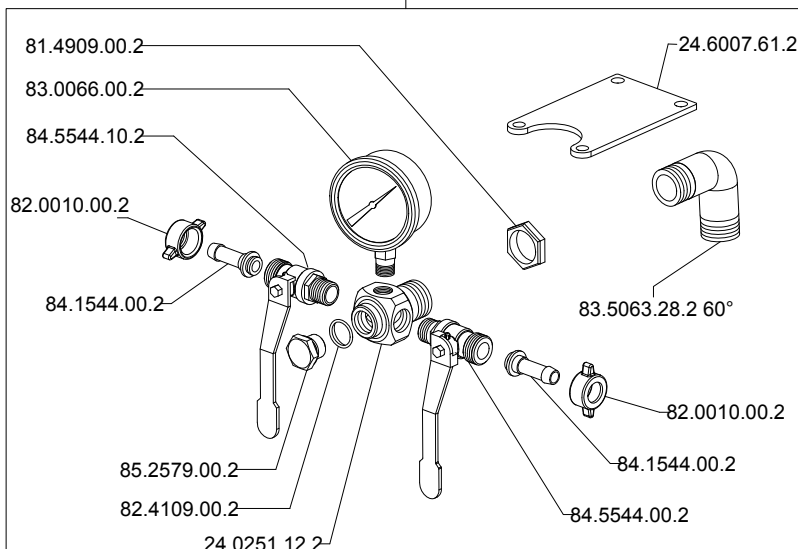
Kit comando a distanza - Remote mounting kit 24.6021.97.3
